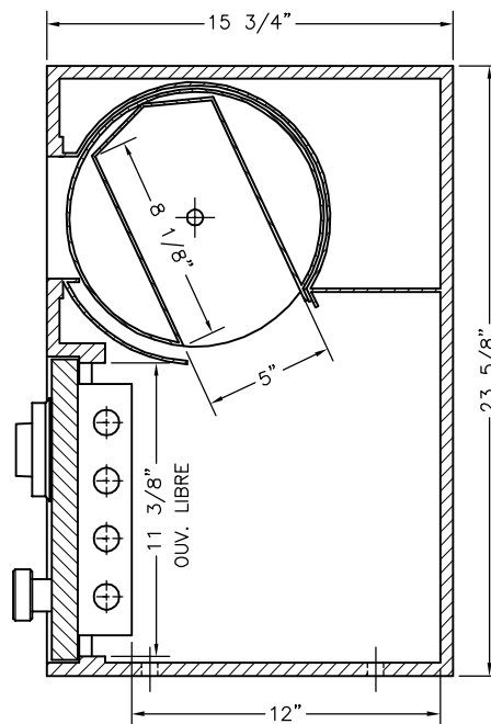
SECTION VERTICALE
