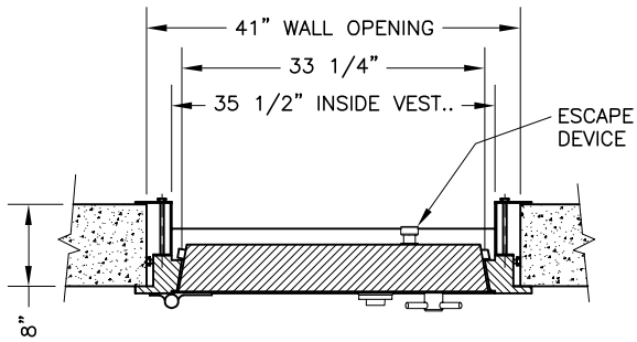
HORIZONTAL CROSS SECTION
